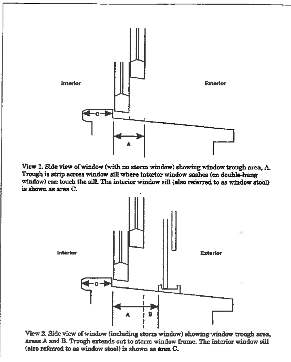
Figure 7-7 Diagram of Building Components
