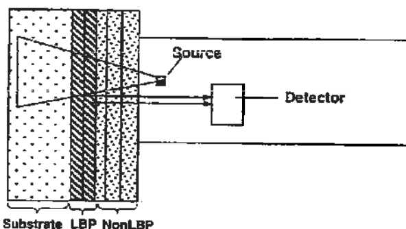
Figure 5-1. XRF emitting gamma and X rays and analyzing characteristic X rays from paint and substrate
