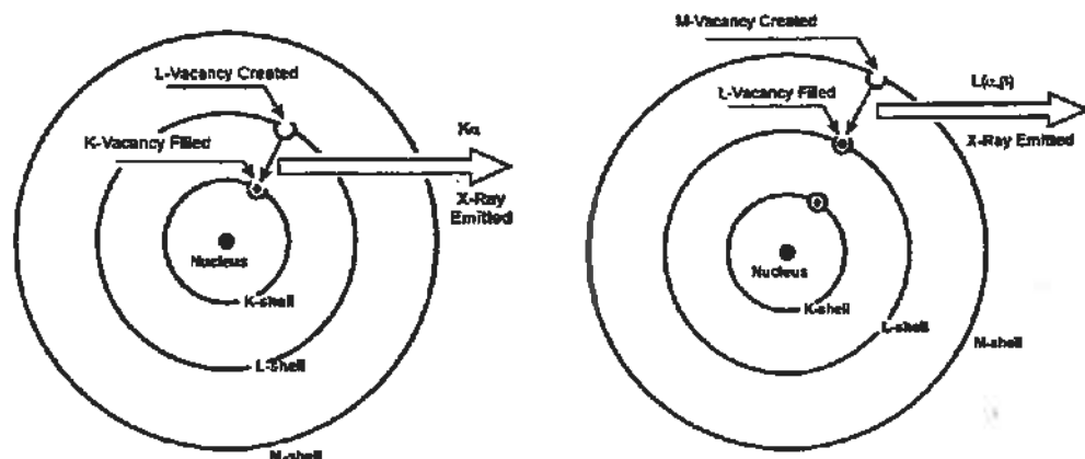
Figure 5-3. Illustration of electron shell vacancies and filling
