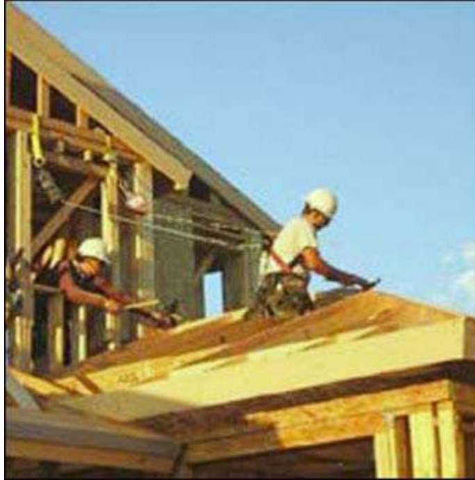
Figure 5 - Strap anchors providing anchorage for three personal fall arrest systems.
